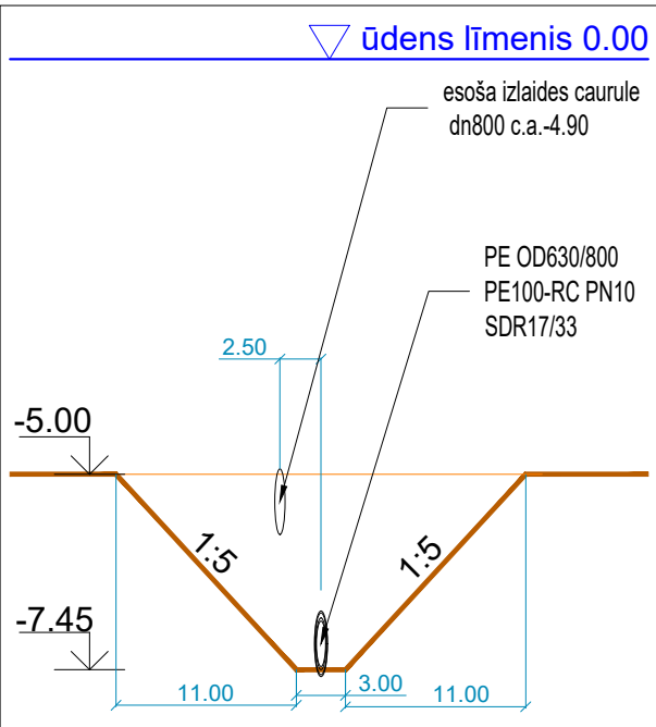
11-11
