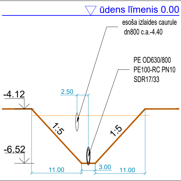
14-14
