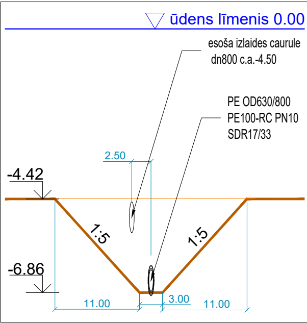
13-13
