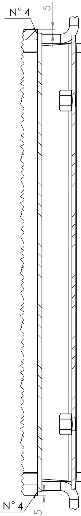
SECTION F-F SCALE 1 : 3
